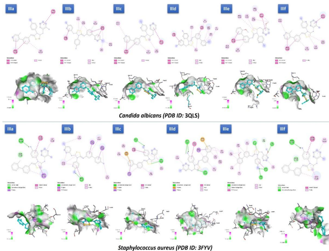
Figure 1. Molecular docking interactions of synthesized dithiazolidine derivatives (IIIa–IIIf) with Candida albicans DHFR (PDB ID: 3QLS) and Staphylococcus aureus DHFR (PDB ID: 3FYV). The top panels show 2D ligand–residue interaction maps, and the bottom panels depict 3D binding poses within the active site pocket. Similarly, IIIc and IIId demonstrated stronger binding to Staphylococcus aureus DHFR (3FYV, −10.3 and −10.8 kcal/mol, respectively) compared with the native ligand (−8.9 kcal/mol). The docking pose of IIId (Figure 2) revealed stable hydrogen bonding interactions and van der Waals contacts, rationalizing its higher docking score and supporting its potent antibacterial potential.
