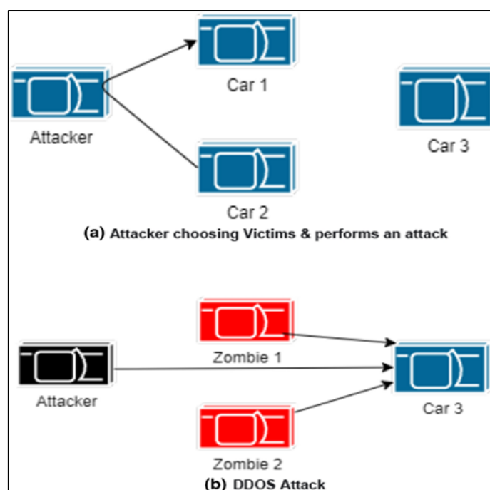
Figure 2: DoS Attack I VANET
